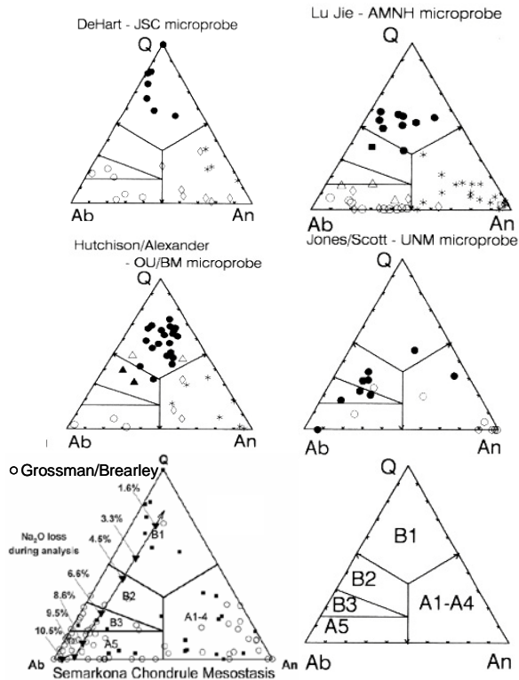
Fig. 3: Ternary diagrams of mesostasis data for DeHart [4] and other sources.
